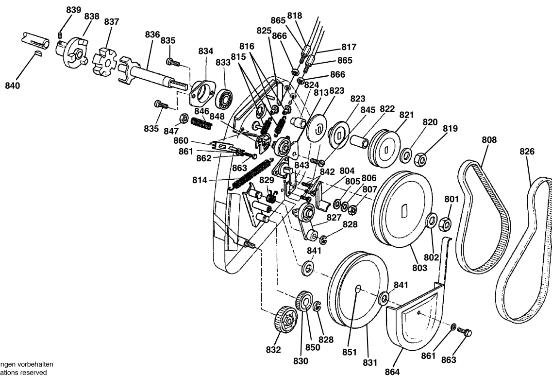
Fig./Abb. 8 FROM SERIAL NUMBER 001699A
