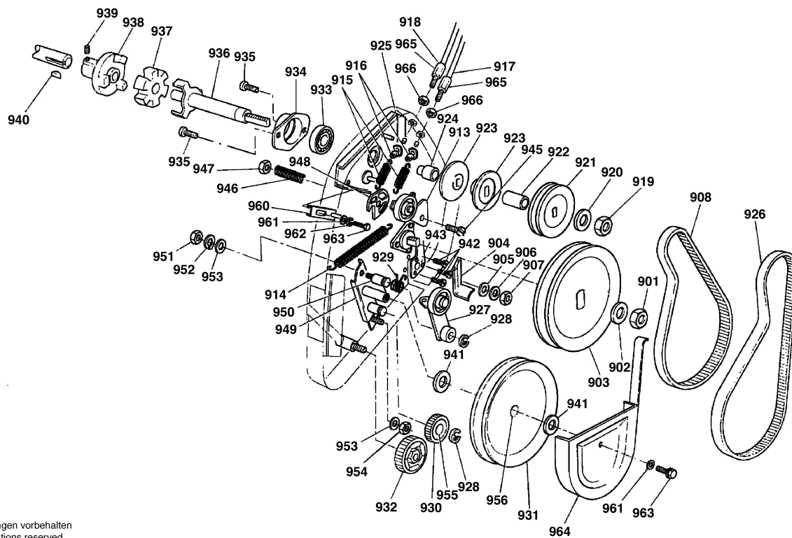
Fig./Abb. 9 FROM SERIAL NUMBER 001892A
