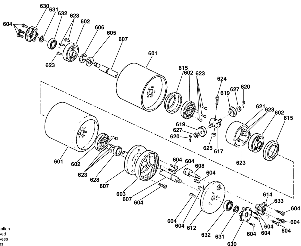
Fig./Abb. 6 FROM SERIAL NUMBER 001892A
