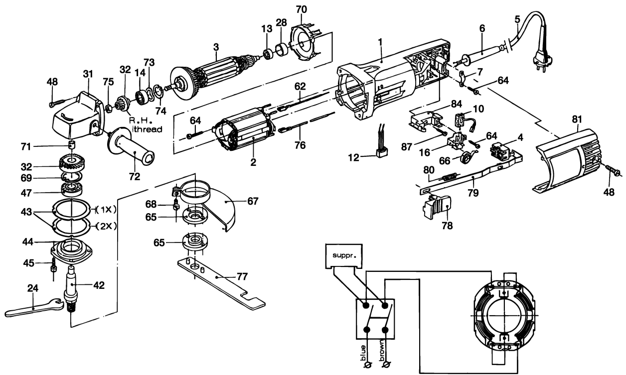
WIRING DIAGRAM
