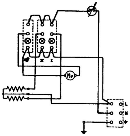
FH 100 WIRING DIAGRAM
