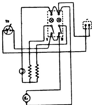
FH 300 WIRING DIAGRAM
