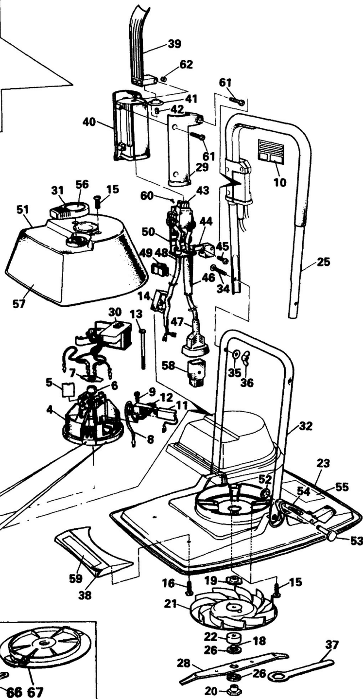
TYPE HX3P - HX3PD
