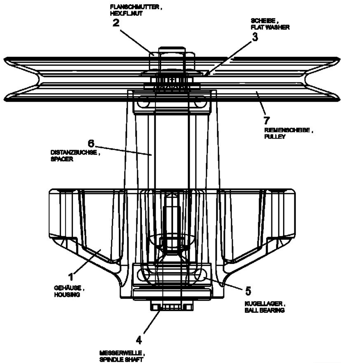
MESSERSPINDEL VOLLST. SPINDLE ASSEMBLY.
