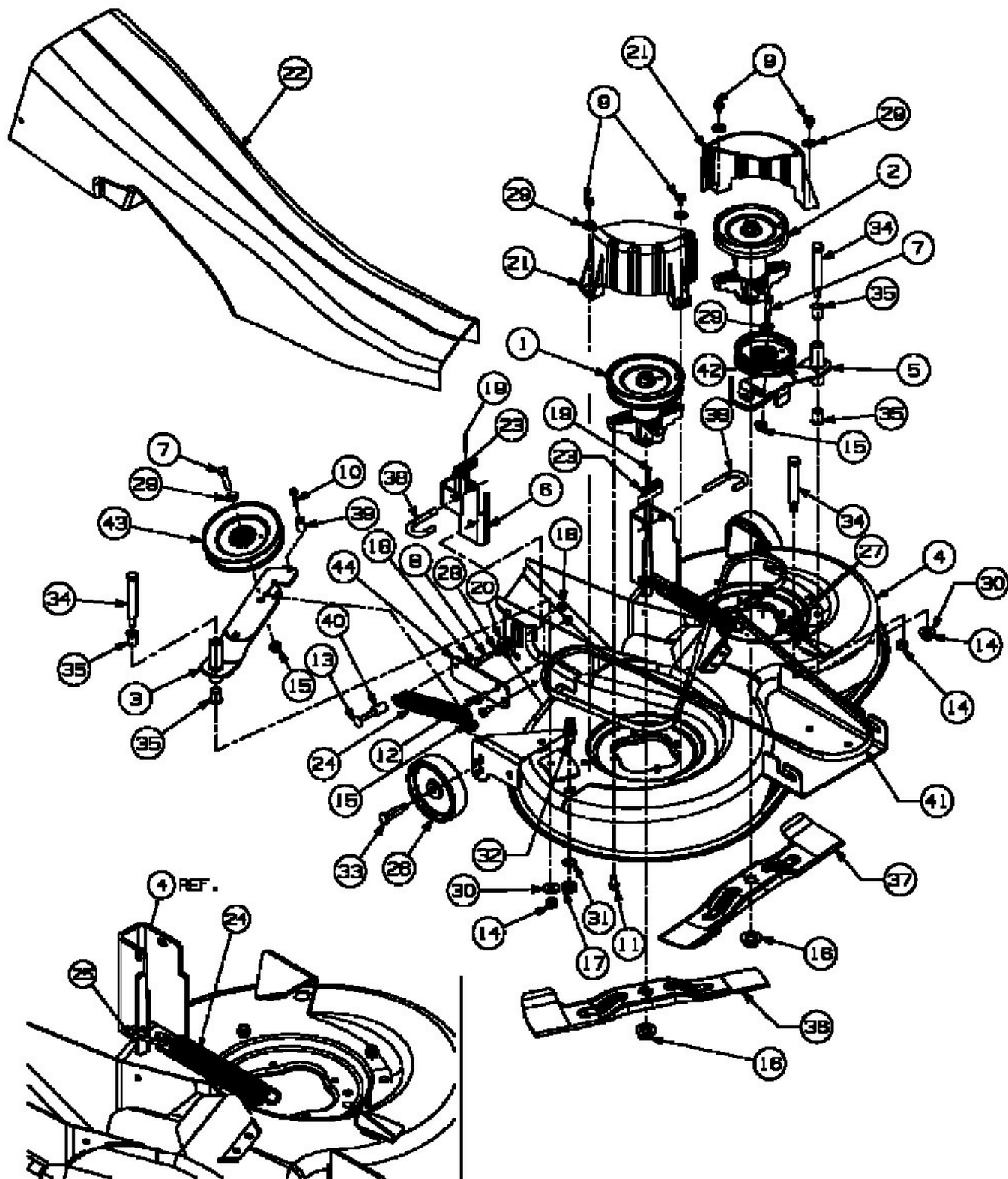
INSTALLATION OF SPRING Feder-Montage
