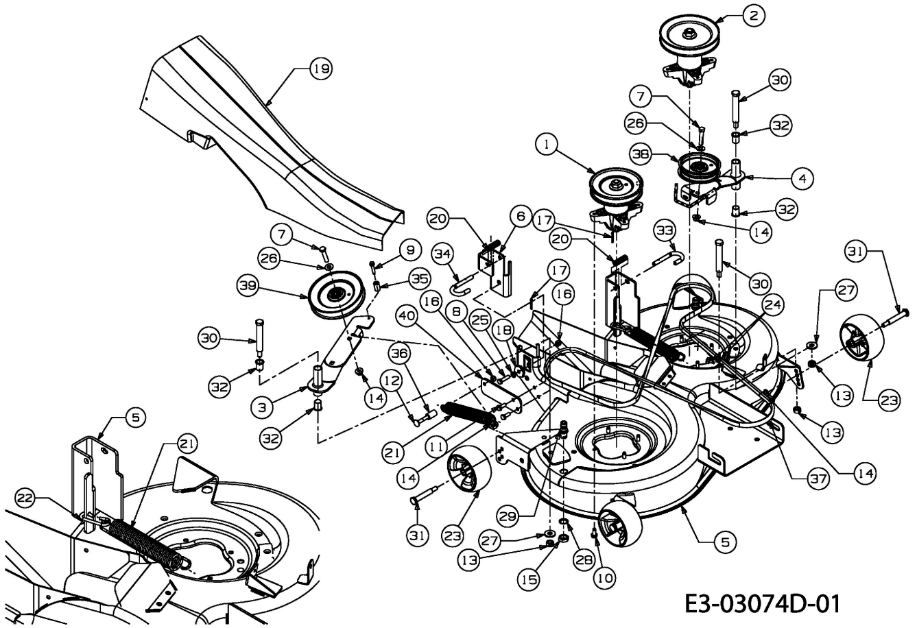
INSTALLATION OF SPRING
